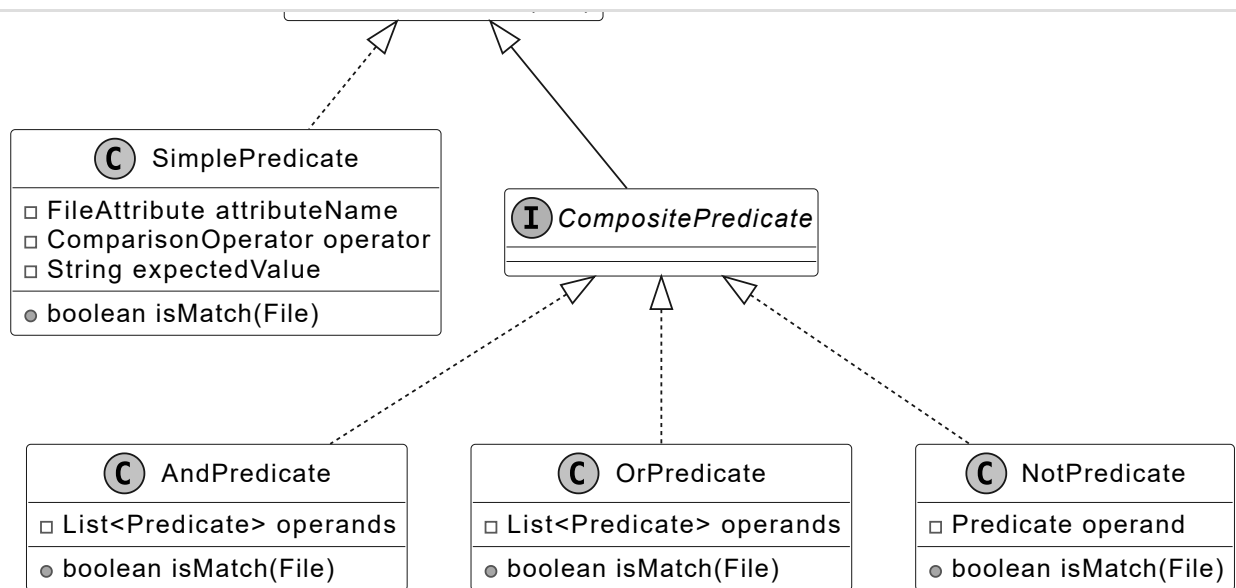
CompositePredicate interface and concrete classes
