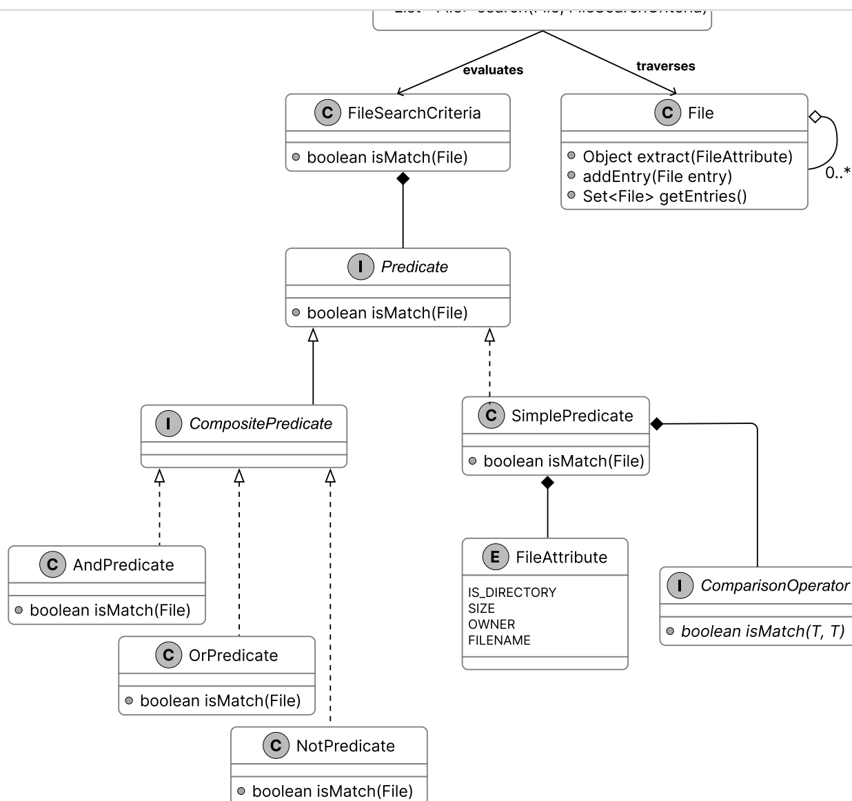
Class Diagram of File Search
